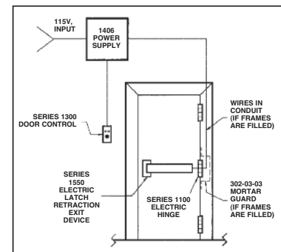
Series 1550 Typical Installation
