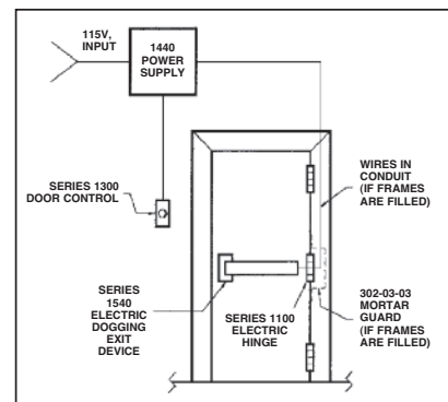
Series 1540 Typical Installation
